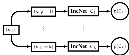
Figure 3: IncNet network for classification.
